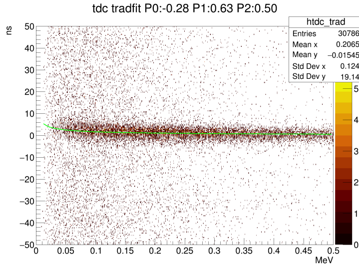
Figure 16: HCal TDC vs E,
