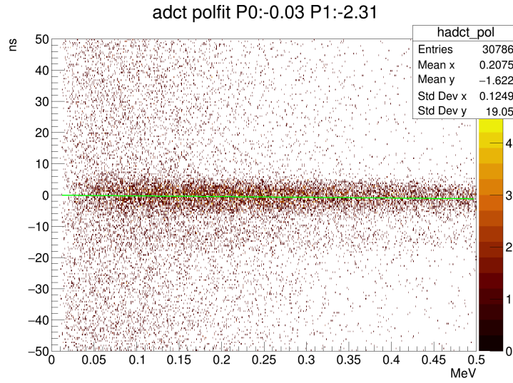
Figure 17: HCal ADCt vs E
