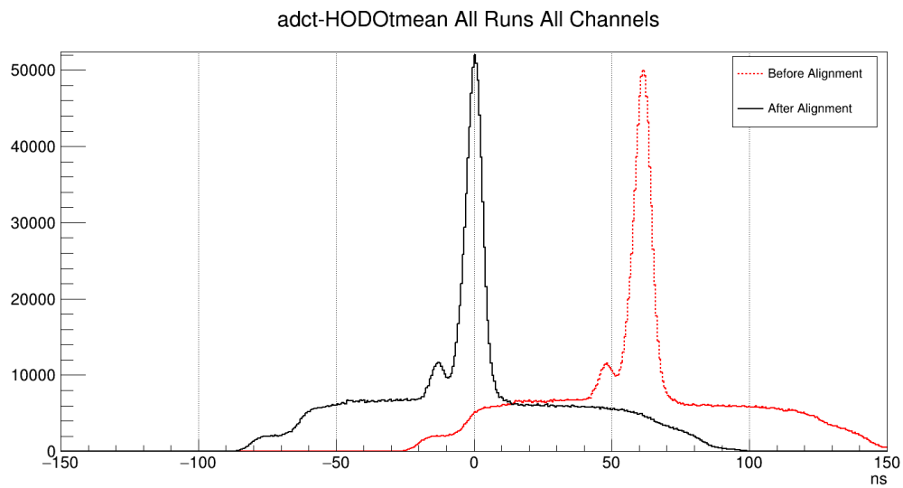
Figure 7: ADCt Comparison, All Channels. Post-alignment Mean: 0.19 ns
