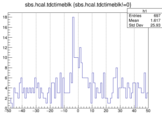
Figure 19: TDC All Channels, Run 12049
