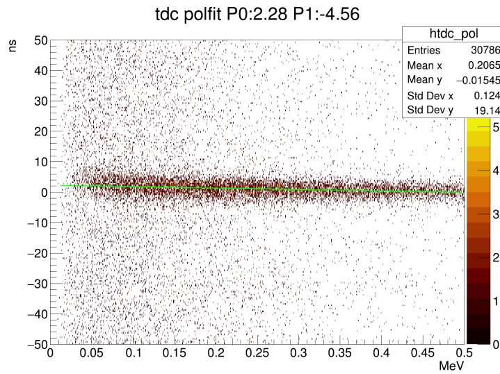
Figure 14: HCal TDC vs E
