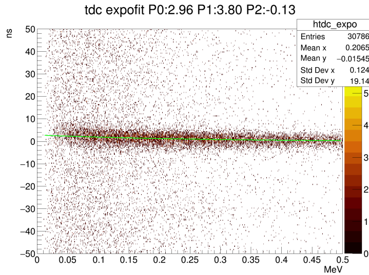
Figure 15: HCal TDC vs E
