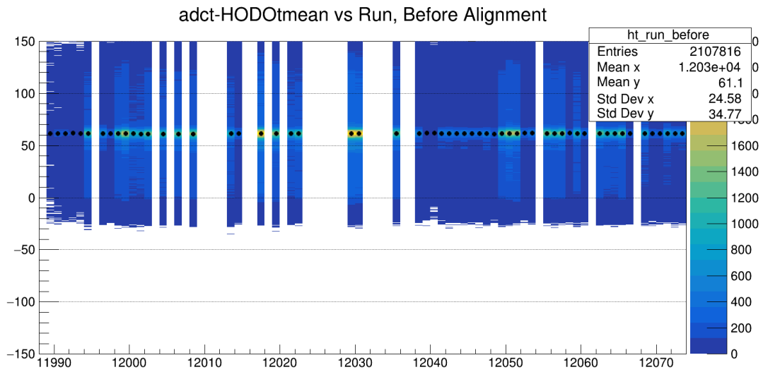
Figure 8: HCal ADCt vs Run Number All Channels, Before Alignment
